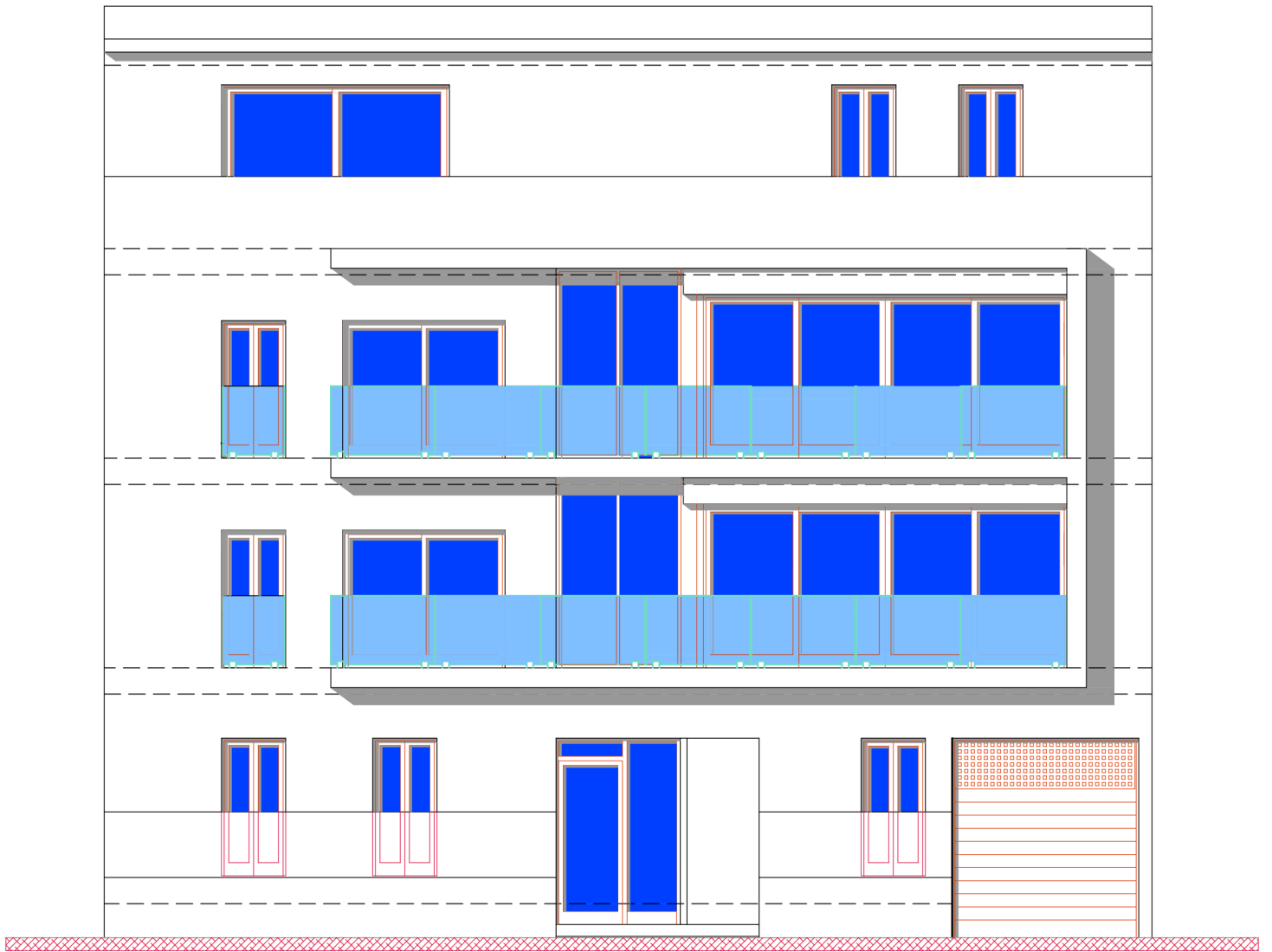
ALZADO PRINCIPAL
